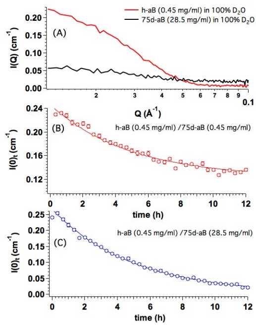
Fig. 1. (a) scattering profiles from crystallin. (b)(c) Subunit dynamics under dilute and crowding system.
